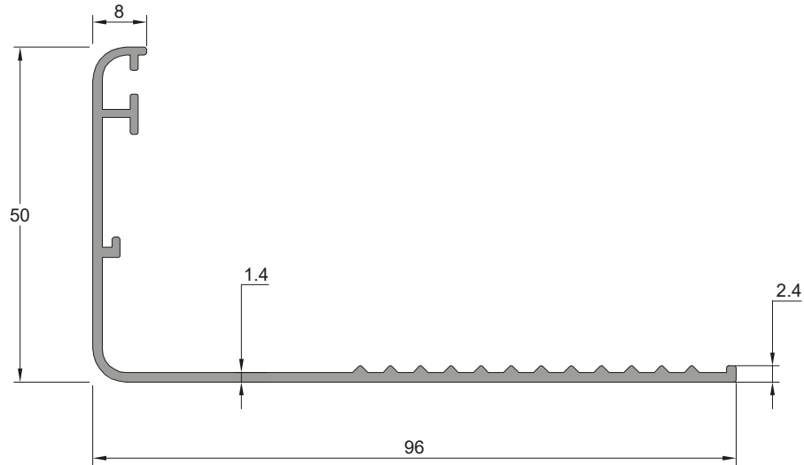
Pervaz Profili SILL PROFILE
