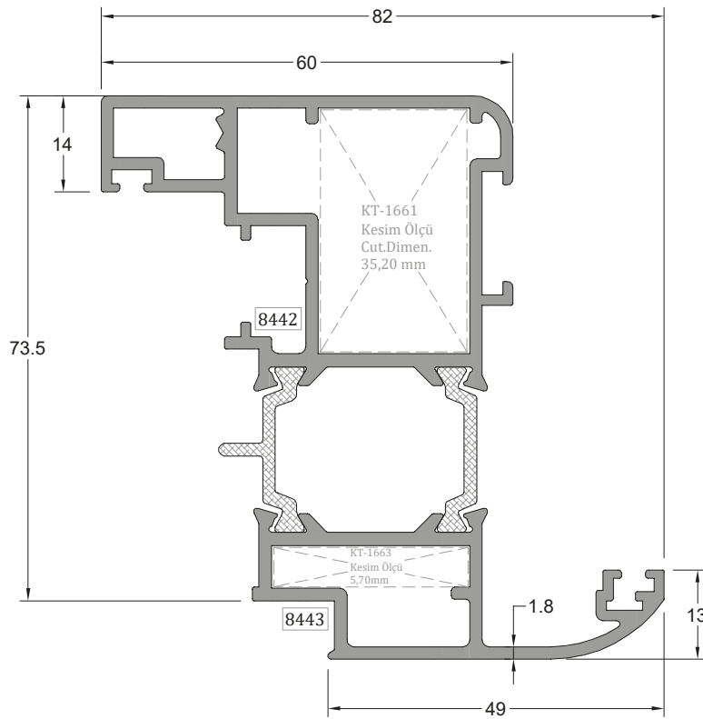
Pvc Kanallı Kanat Profili PVC GROOVE SASH PROFILE
