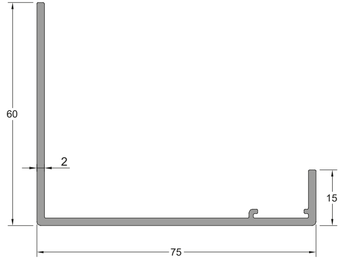
Pervaz Profili SILL PROFILE
